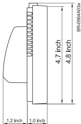
USG-4000: Power module for large applications.
